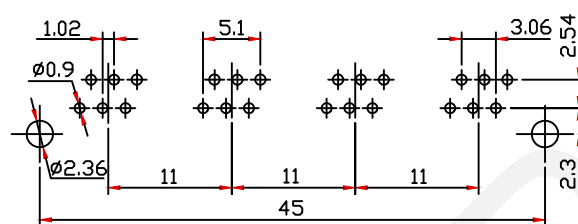
PCB Layout
